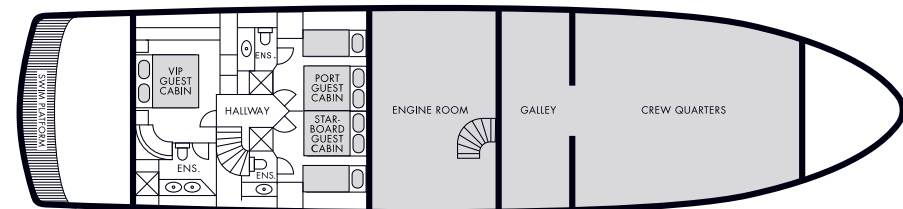
CABIN DECK
